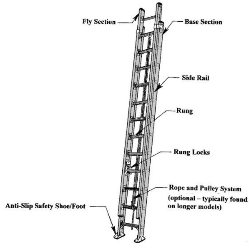
Extension Ladder
